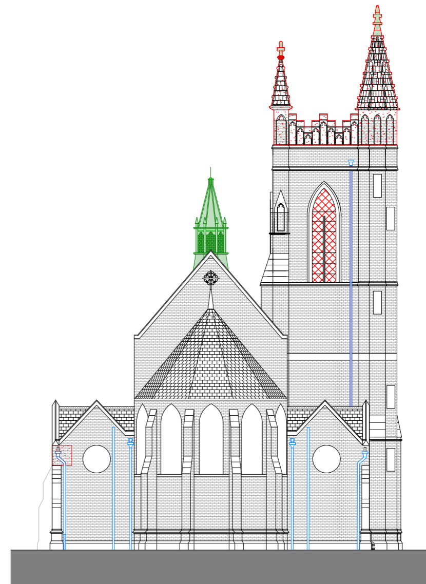
Scope of Work, East Elevation, 1:200
